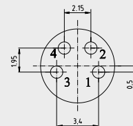
Buchse M8 x 1, 4-polig
