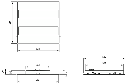
RC342B LED36S/940 PSD W62L62 VPC PCS
