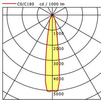
Flixx 200 Round (FLIRZ 200.25, 1xLED 27W 830/3000K 2890lm 15 °)
