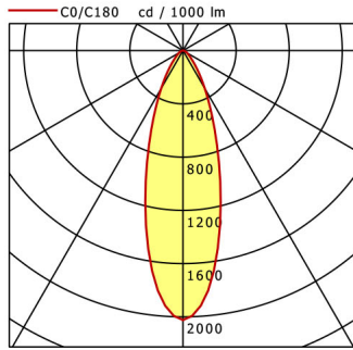
Flixx 200 Round (FLIRZ 200.05, 1xLED 27W 830/3000K 2970lm 15 °)
