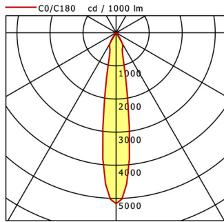
Flixx 100 Round (FLIRZ 100.25, 1xLED 15W 827/2700K 1270lm 15 °)
