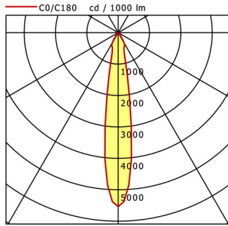
Flixx 100 Round (FLIRZ 100.24, 1xLED 15W 827/2700K 1230lm 15 °)
